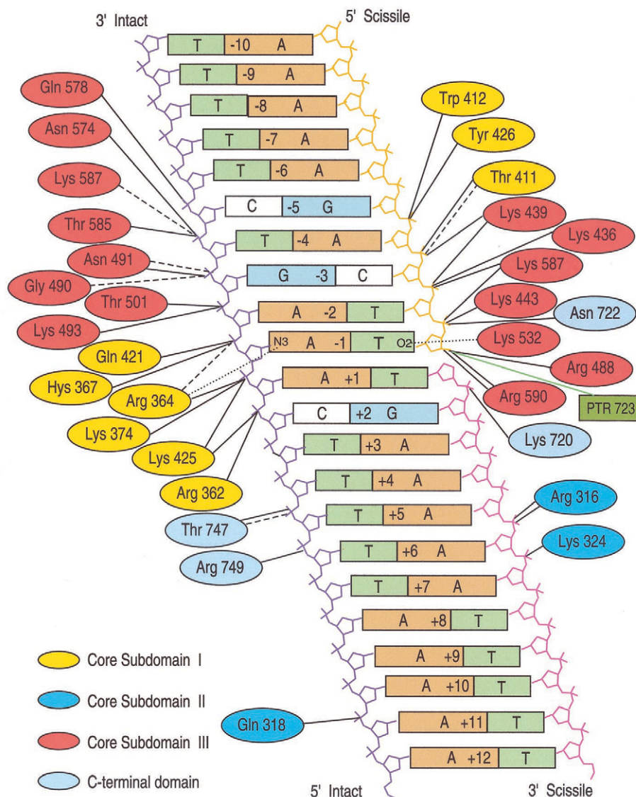
FIGURE 2A Schematic representation of the protein-DNA direct ( a ) and water-mediated ( b ) interactions present for more than 70% of the simulation time. Full line , protein side chain-DNA phosphate group; dashed line , protein main chain-DNA phosphate group; dotted line , protein side chain-DNA base atoms; dash-dotted line , protein main chain-DNA base atoms. The phosphotyrosine bond is represented by a full green line. Different colors refer to different protein domains. ( b ) Thick and thin lines represent long life and fast exchanging waters, respectively.
