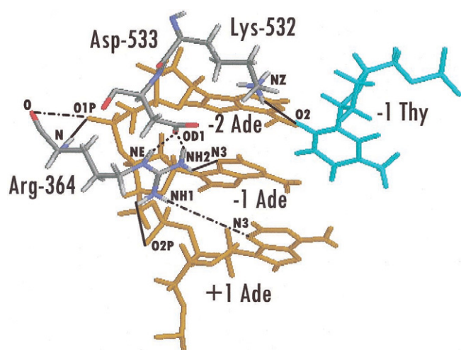
FIGURE 4 Network of direct and water-mediated interactions between Arg364 and DNA. The three direct hydrogen bonds with the DNA-intact strand (N3 atom of the -1 adenine base and the phosphate groups of the -1 and -2 adenine bases) are represented by full lines ; the two water-mediated hydrogen bonds with the DNA-intact strand (N3 atom of the +1 adenine base and phosphate groups of -2 adenine base) are represented by dash-dotted lines ; the two direct hydrogen bonds with Asp533 (OD1 atom) are represented by dotted lines . In the figure is also represented the direct hydrogen bond between Lys532 and the -1 thymine base (O2 atom) by a full line . The three bases of the DNA intact strand and the scissile base are represented in yellow and cyan , respectively.
